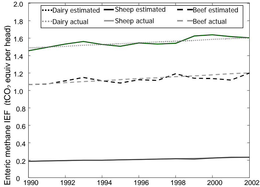
Figure 2: Implied emission factors—actual and estimated
