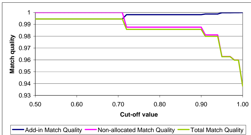
Figure 2: 1991 match quality of TA to RC, varying cut-off
